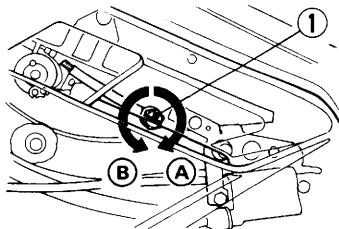
(1) Throttle stop screw (A) Increase (B) Decrease
